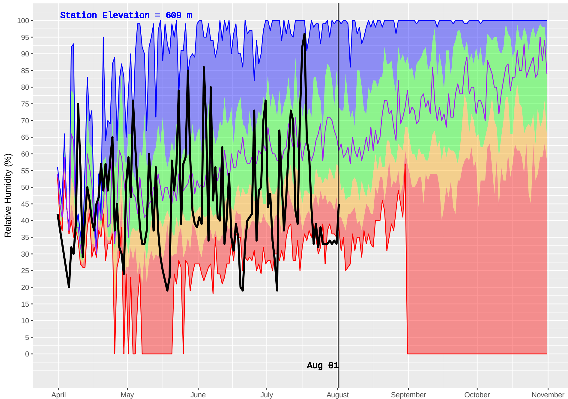
BOB QUINN LAKE (113) : Historical (1984–2016) and Current (2018) Daily Relative Humidity
